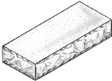
ROCK FACE Heavy relief, hand cut (chiseled) edges, thermal top, sawn backs.
